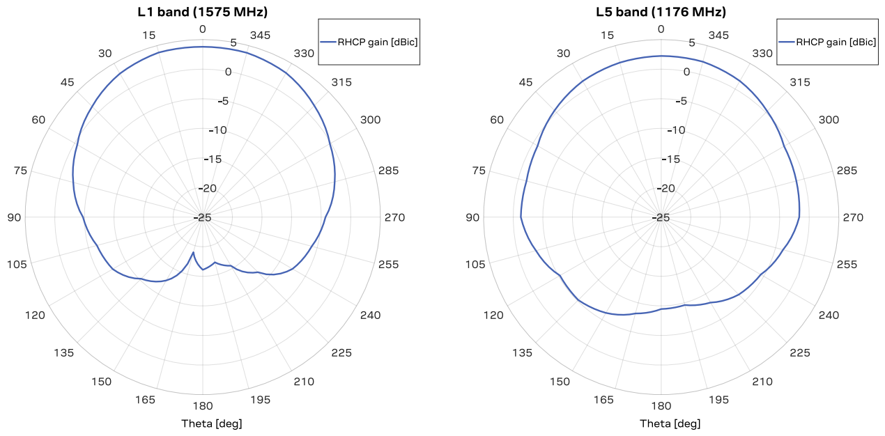
Figure 1: E plane ( \phi = 0 ) radiation pattern at the L1 (1575 MHz) and L5 (1176 MHz) bands measured over a 70 x 70 mm 2 ground plane. Theta = 0 degrees is in the vertical direction.
