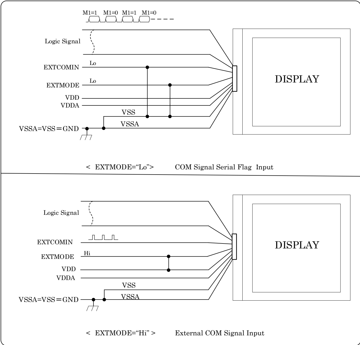
Figure 4-2-1 Recommended circuit
