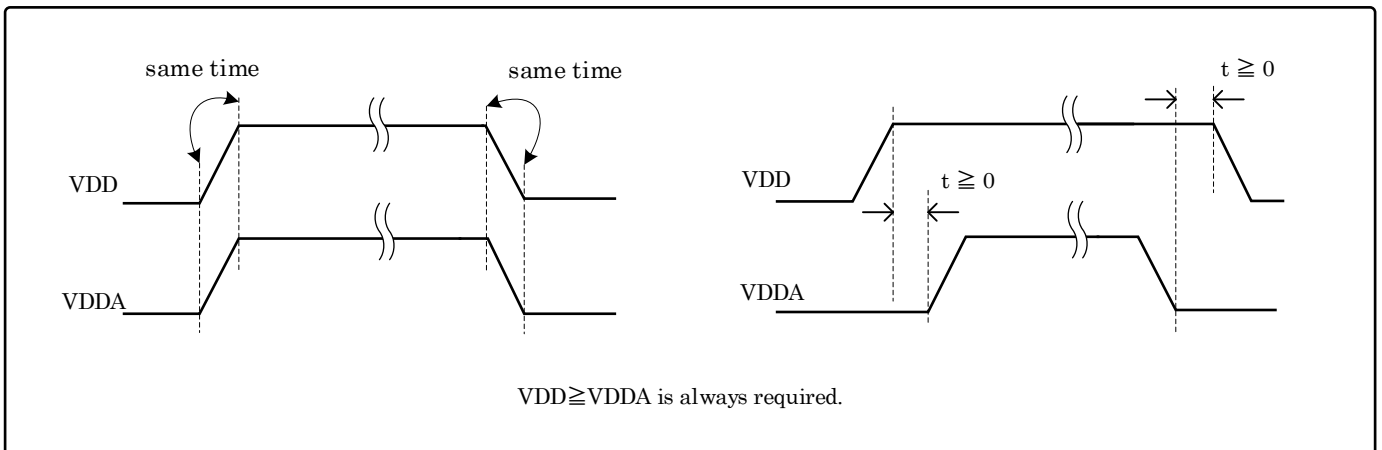
Figure 6-2-2 Power supply sequence
