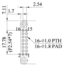
PIN DETAIL
