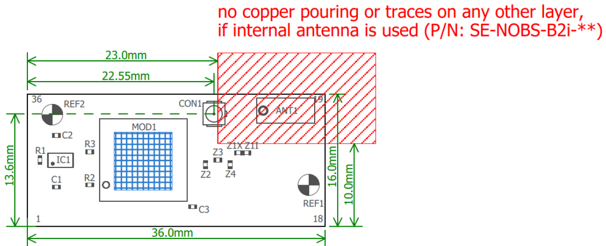
Figure 6 – mechanical information LVIV-B2
