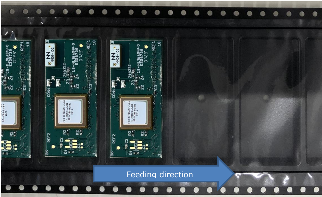
Tap and Reel Orientation of LVIV-B2
