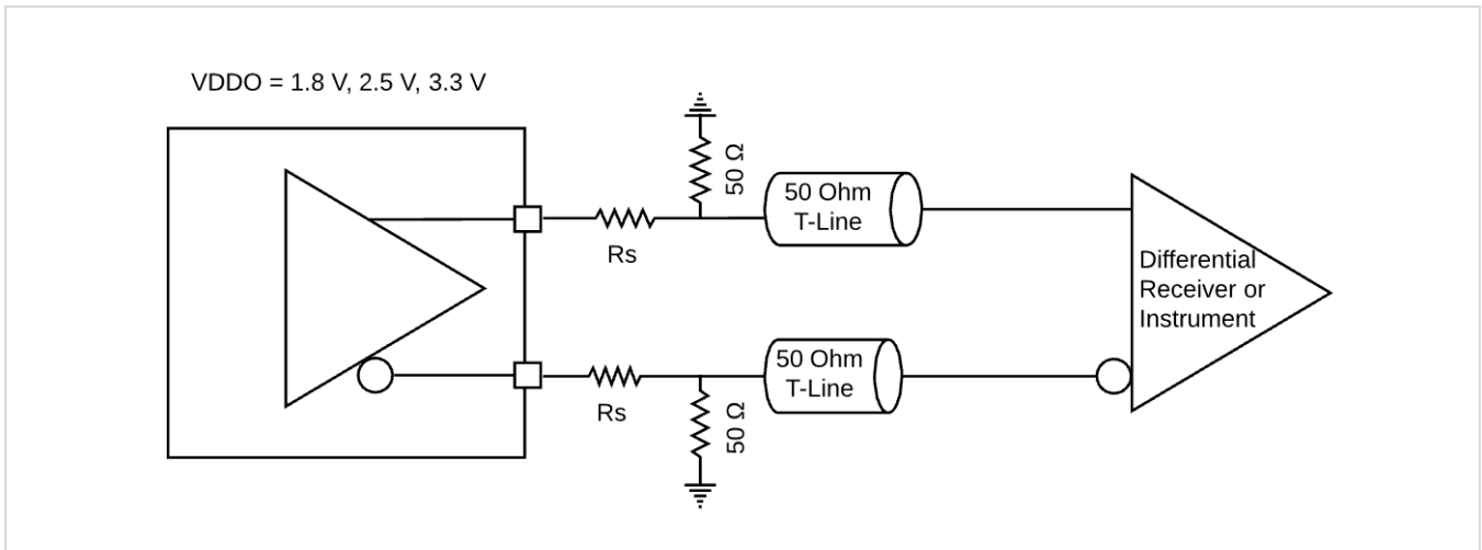
Figure 30. HCSL Interface Termination [51]
