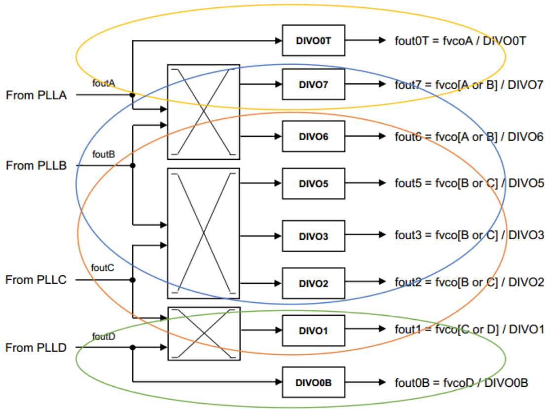
Figure 13. Output Clock Distribution
