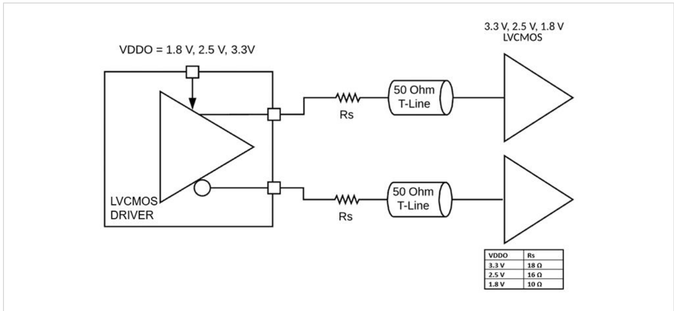
Figure 32. LVCMOS output Termination
