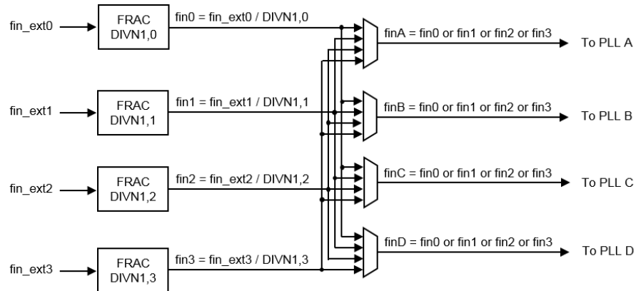
Figure 12. Input Clock Distribution
