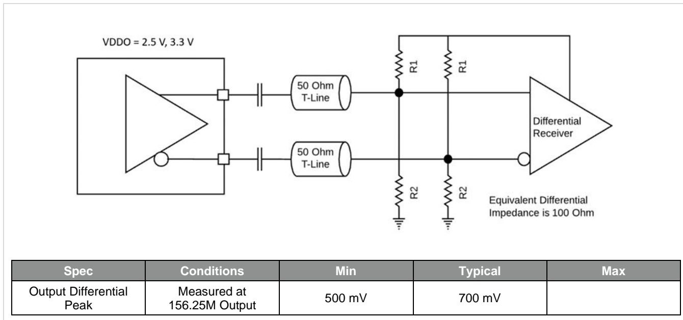
Figure 29. LVDS Boost Standard for the SiT95147 Output Driver with AC Termination at the Load
