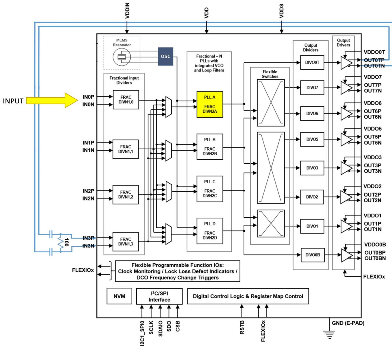
Figure 33. SiT95147 Zero Delay Mode Setup
