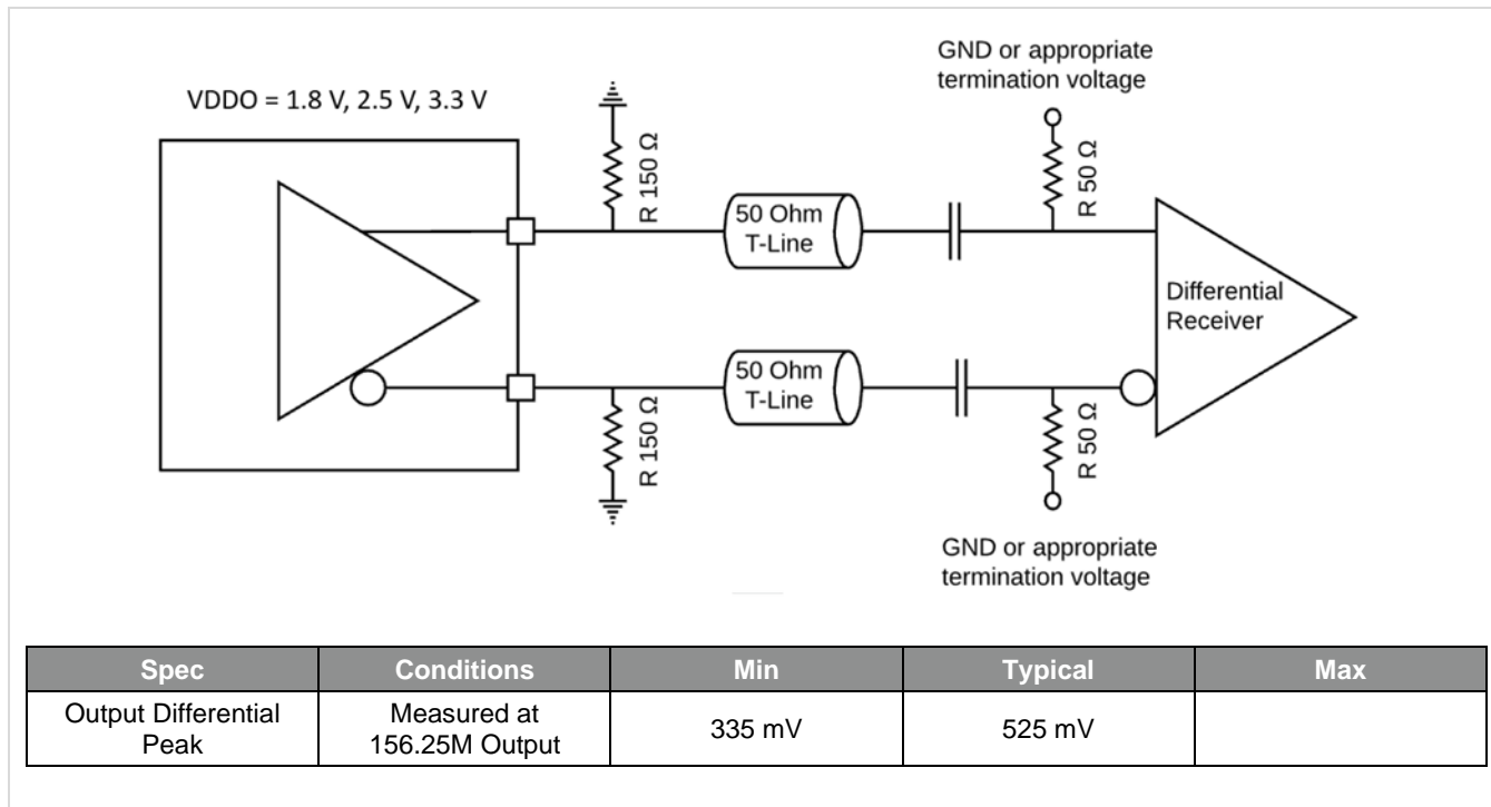
Figure 26. LVPECL2 for the SiT95147 Output Driver with AC Termination at the Load
