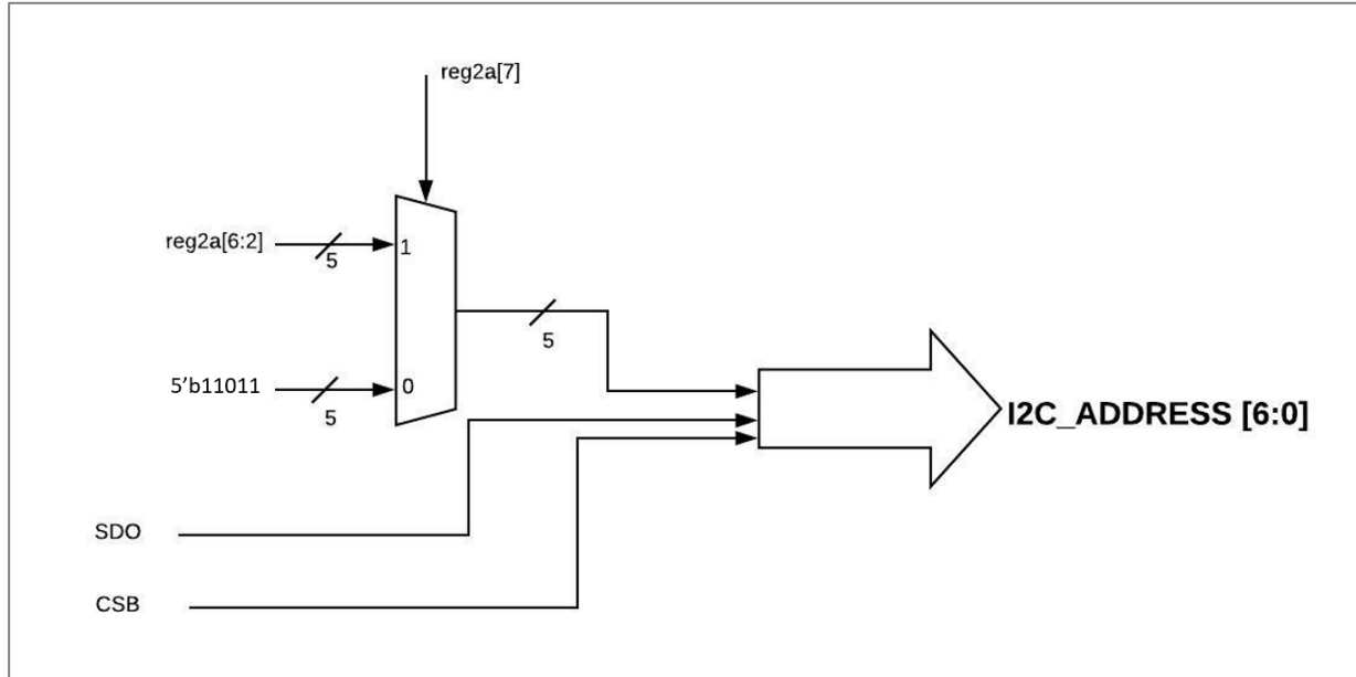
Figure 36. I 2 C Addressing Scheme for Cascade
