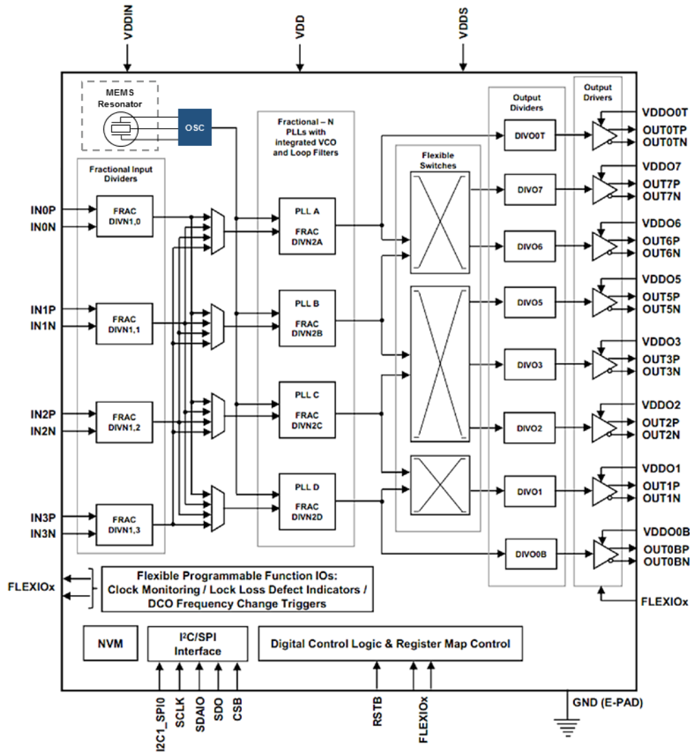
Figure 10. Overall Architecture
